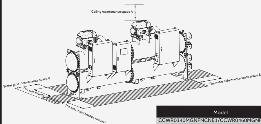
Service space requirements
