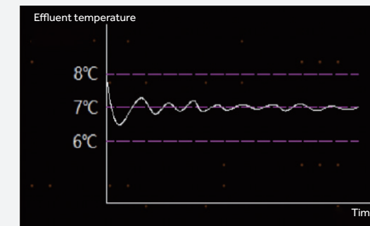
PID control water outlet temperature curve
