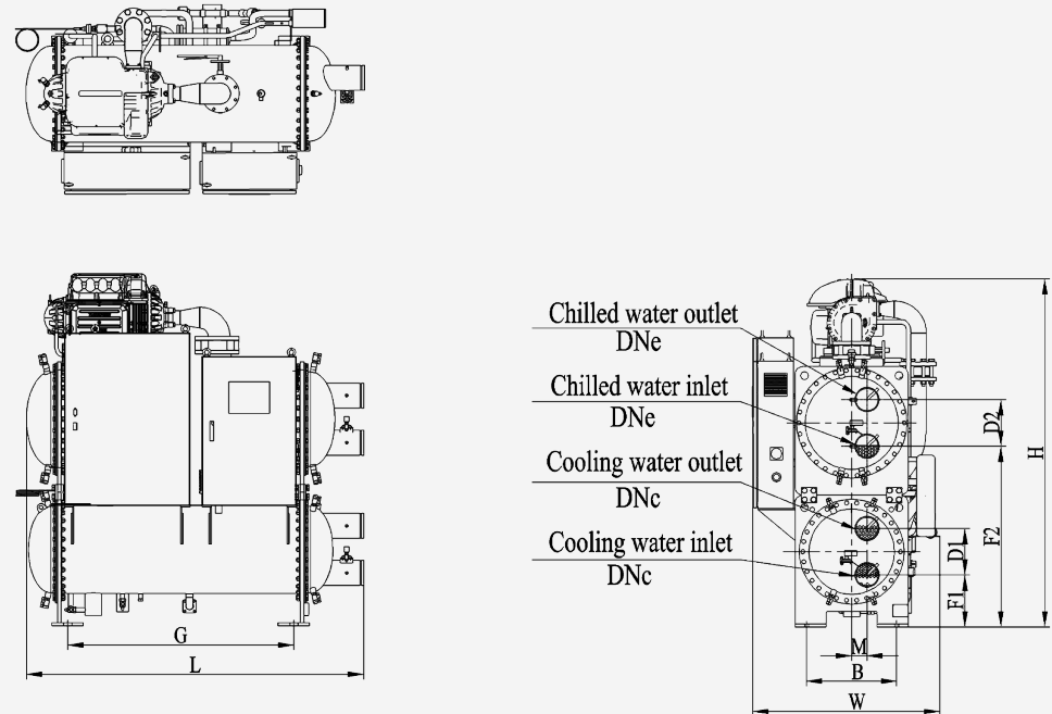
Outline dimension
