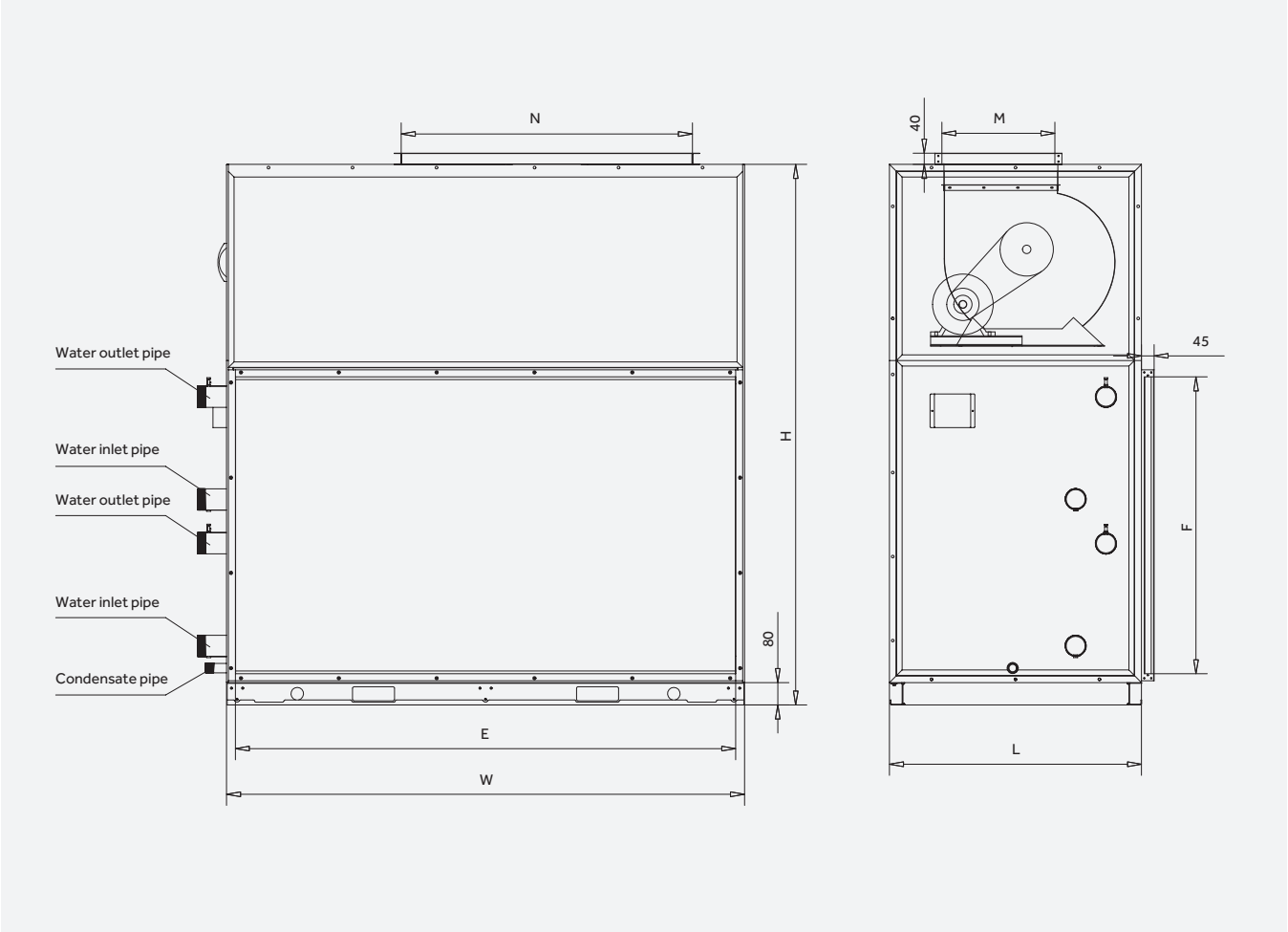
Vertical air handling unit dimension
