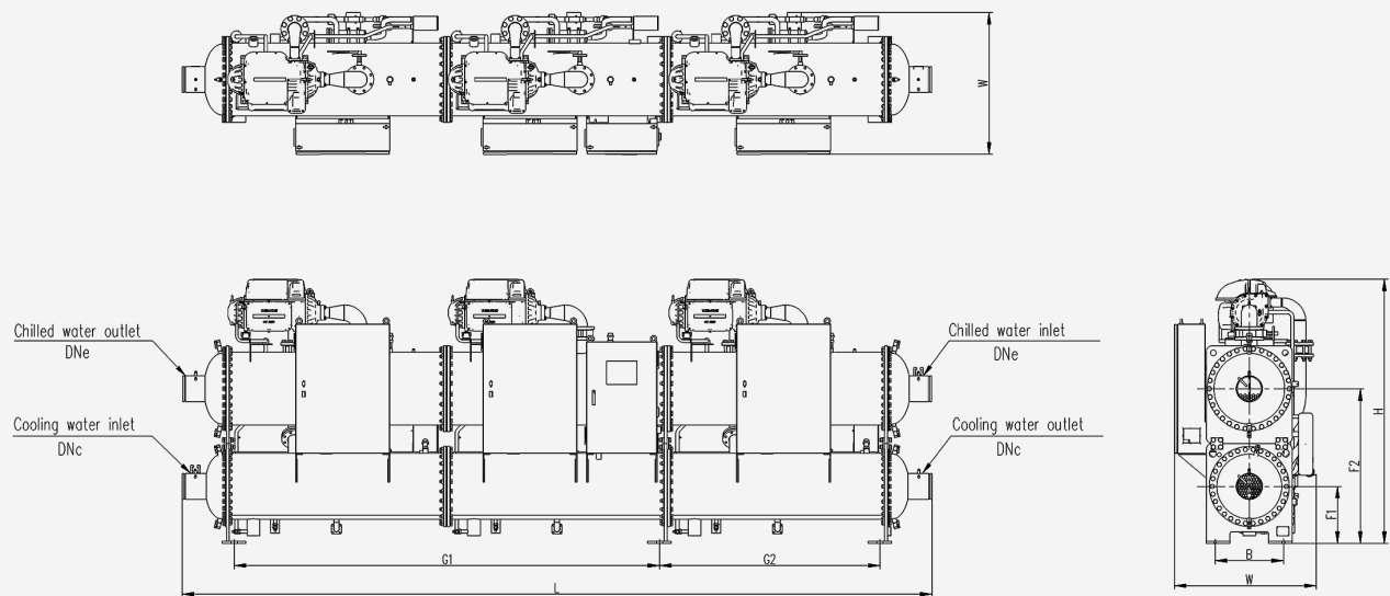
Outline dimension
