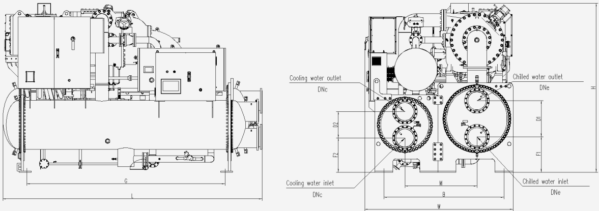
Outline dimension
