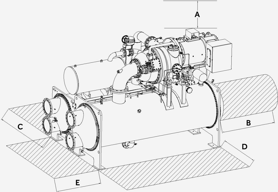
Service space requirements
