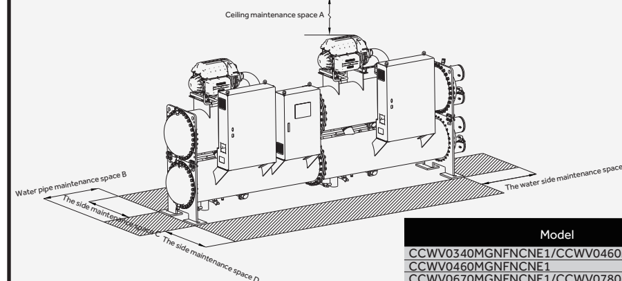
Service space requirements
