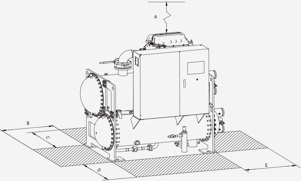
Space diagram
