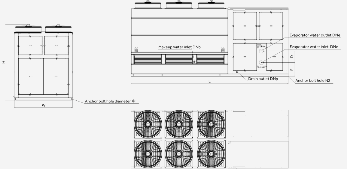
CC0440PENI ~ CC0530PENI Unit dimension
