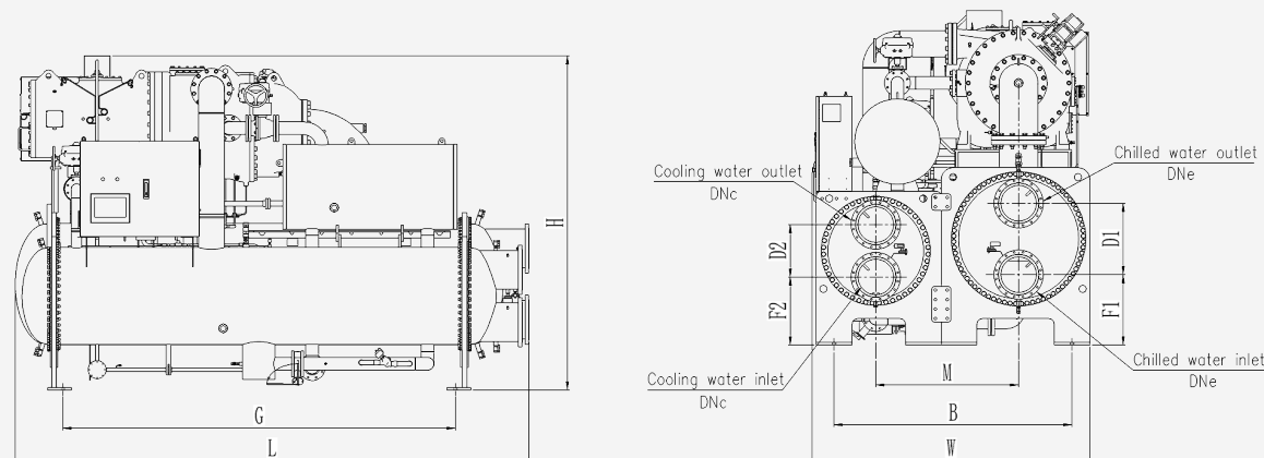
Outline dimension
