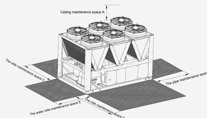
Air-cooled magnetic bearing centrifugal chiller installation space diagram
