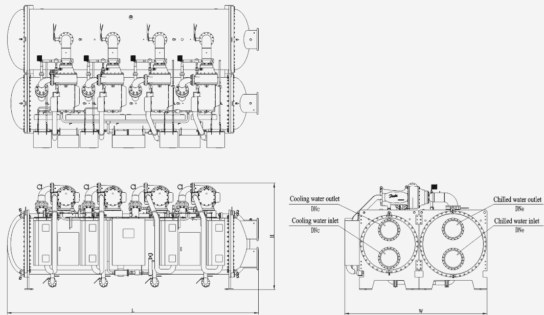
Outline dimension
