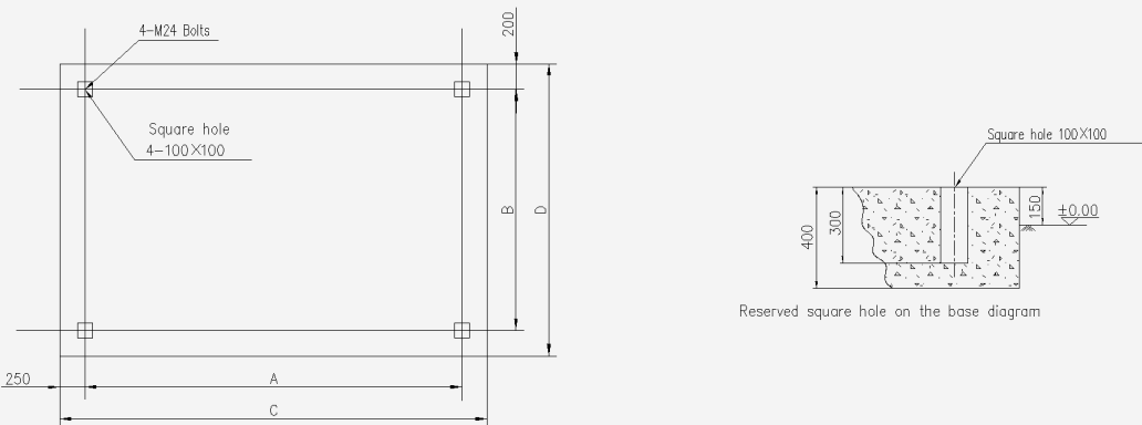
Installation foundation drawing
