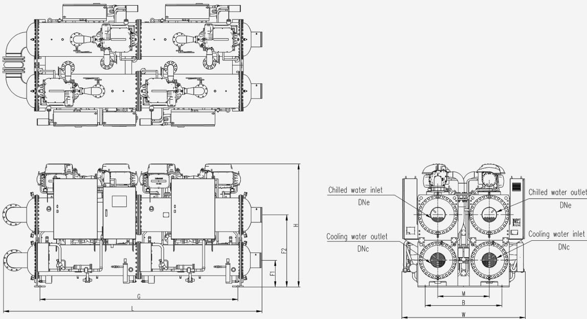
Outline dimension
