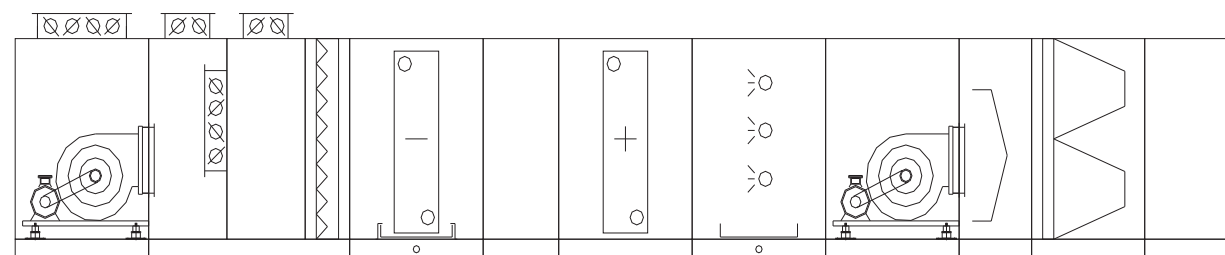
Horizontal Combination 6: Return air fan + fresh air and exhaust air + plate filter+ chilled water coil + middle section + heating coil + humidifier + fan + diffuser + bag filter + air supply
