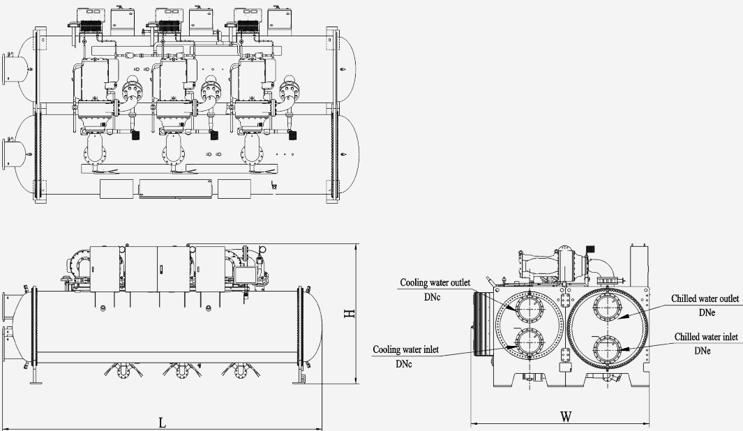
Outline dimension
