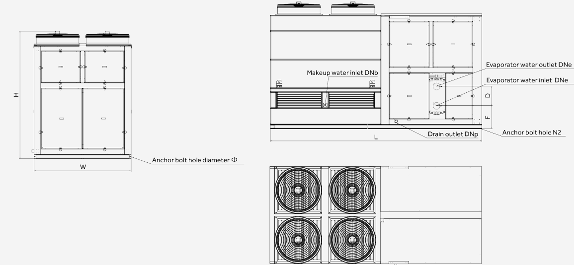
CC0325PENI Unit dimension
