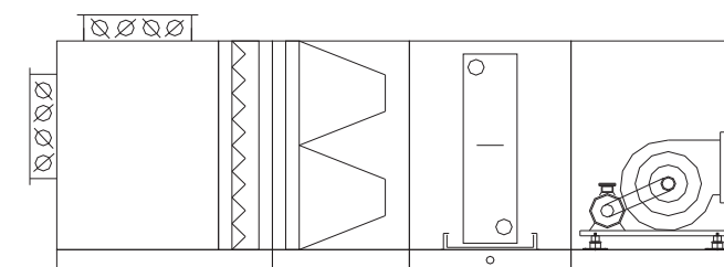
Horizontal Combination 2: Mixing box + bag filter + chilled water coil + fan
