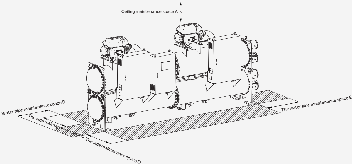
Water-cooled magnetic bearing centrifugal chiller installation space diagram
