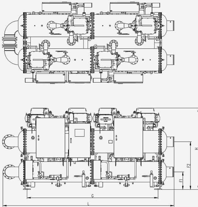
Outline dimension
