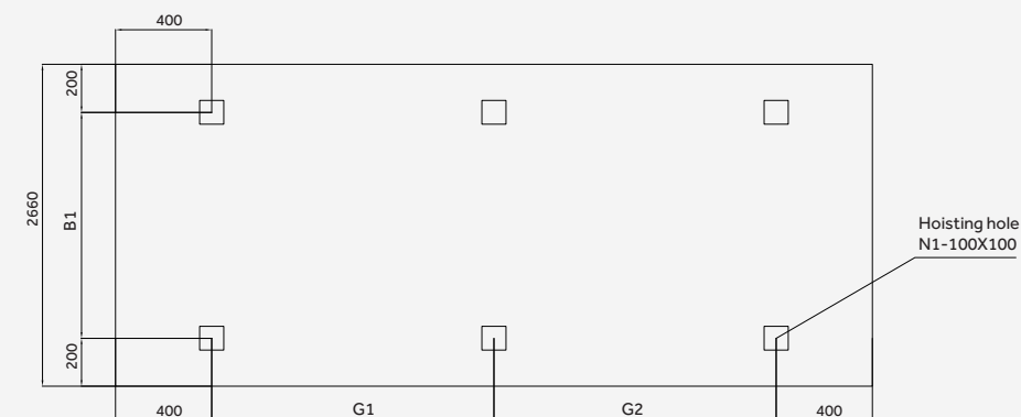
Installation foundation drawing
